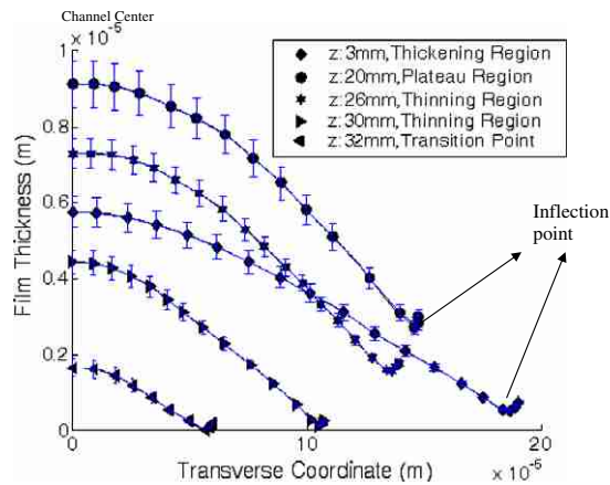
Fig. 7. Cross-sectional profile of liquid film in channel #2 ( G = 89.3 kg/m 2 /s).
