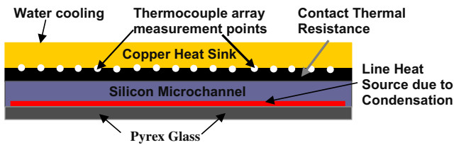
Fig. 16. Microchannel structure schematic.
